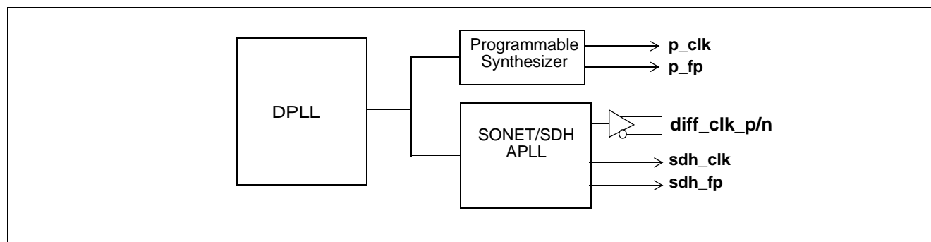
Figure 6 - Output Configuration
