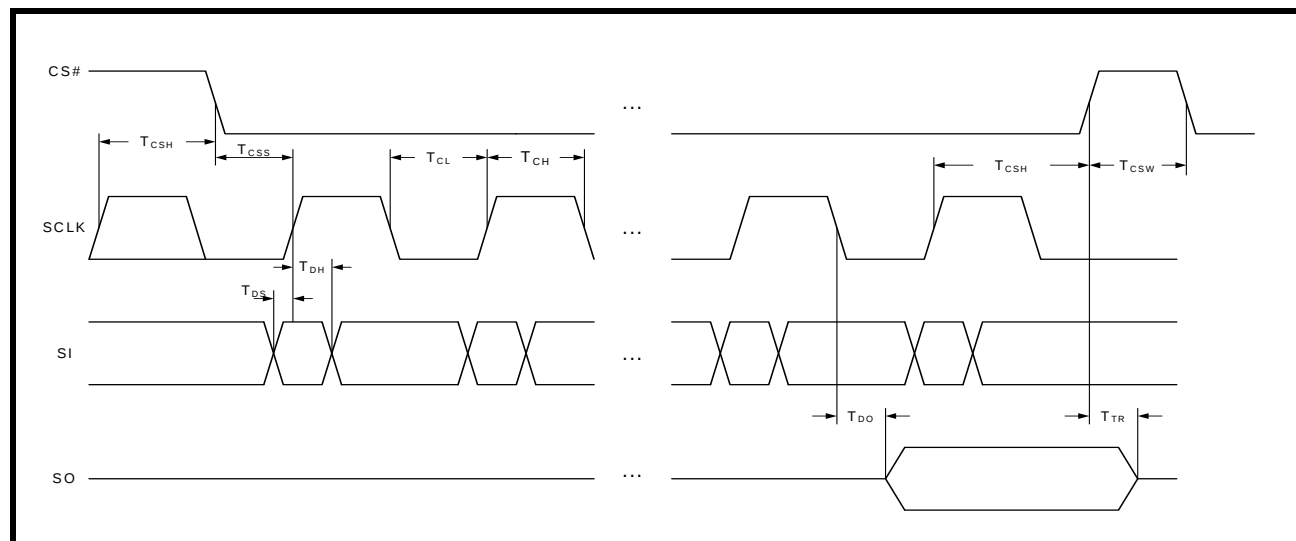
FIGURE 29. SPI-BUS TIMING
