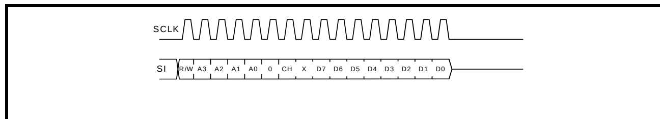
FIGURE 7. SPI WRITE
