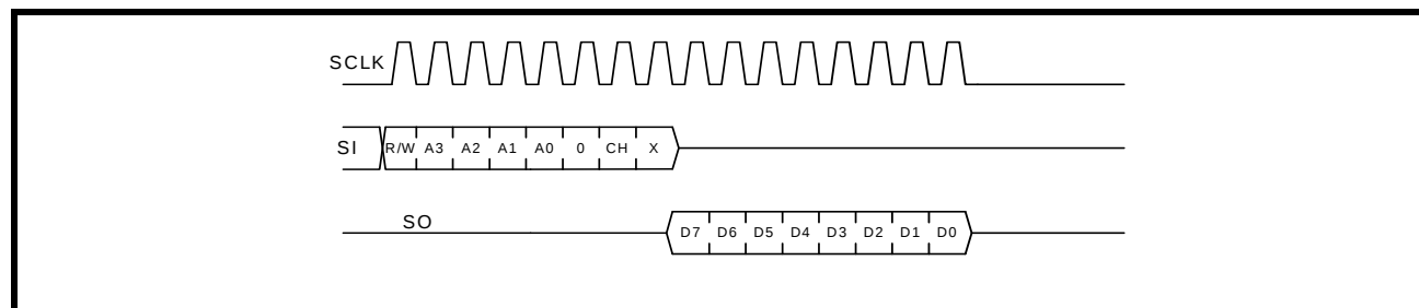
FIGURE 8. SPI READ
