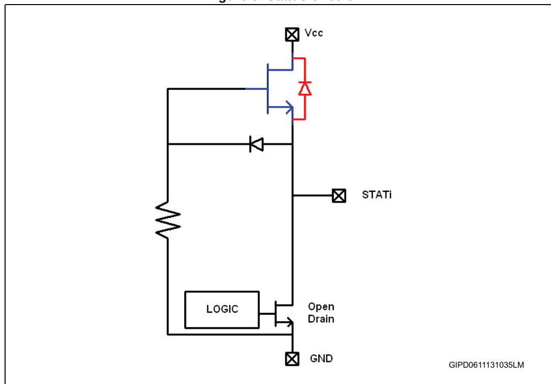
Figure 8. Status circuit
