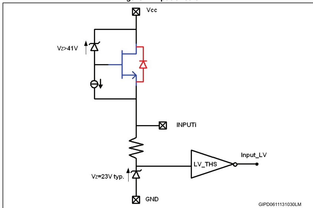
Figure 7. Input circuit
