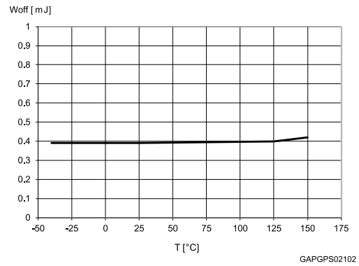
Figure 30: W_{off} vs. T_{case}
