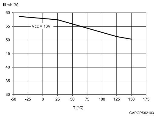
Figure 31: I_{limH} vs. T_{case}
