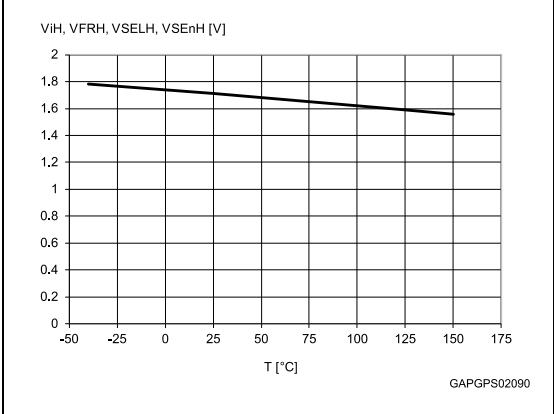
Figure 18: Logic Input high level voltage
