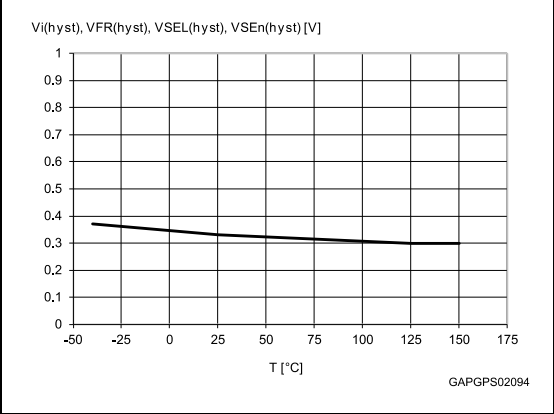
Figure 22: Logic Input hysteresis voltage
