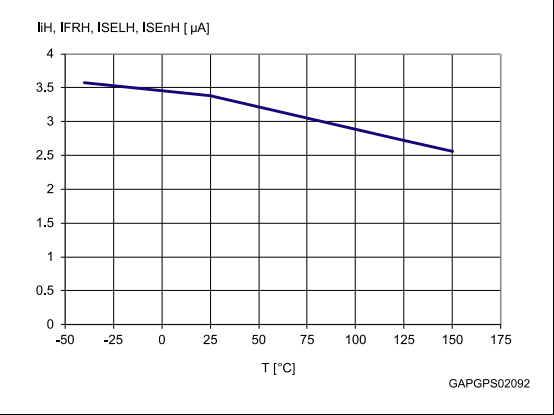
Figure 20: High level logic input current
