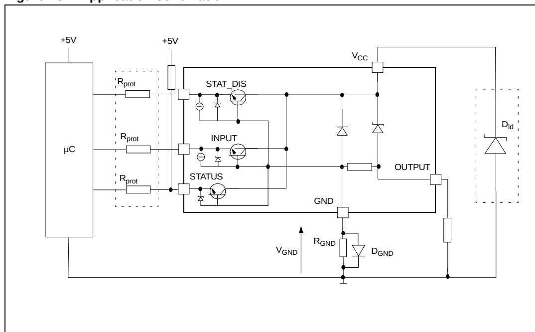
Figure 28. Application schematic
