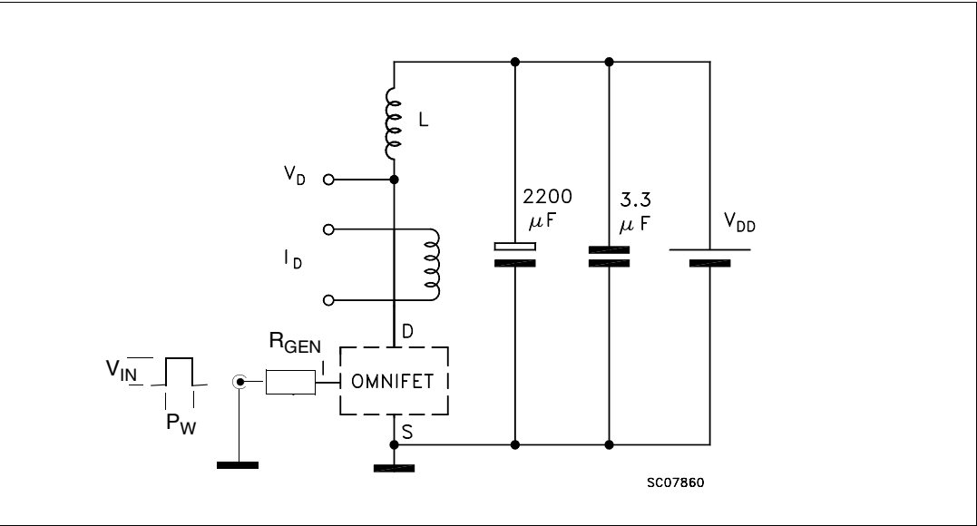
Figure 5. Unclamped inductive load test circuits
