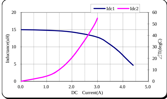
TDK' PartNo.;VLS6045EX-150M
