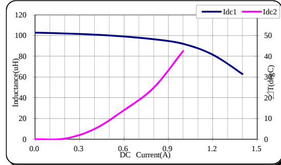
TDK' PartNo.;VLS6045EX-101M
