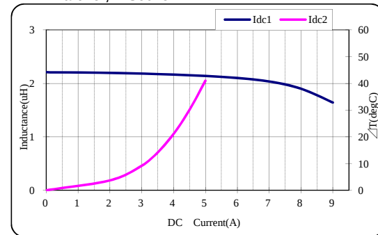
TDK' PartNo.;VLS6045EX-2R2N
