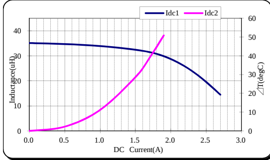
TDK' PartNo.;VLS6045EX-330M
