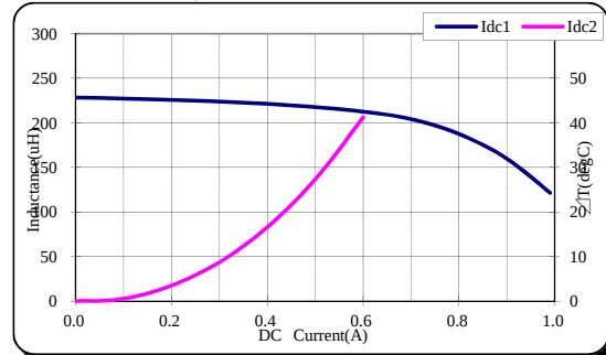
TDK' PartNo.;VLS6045EX-221M
