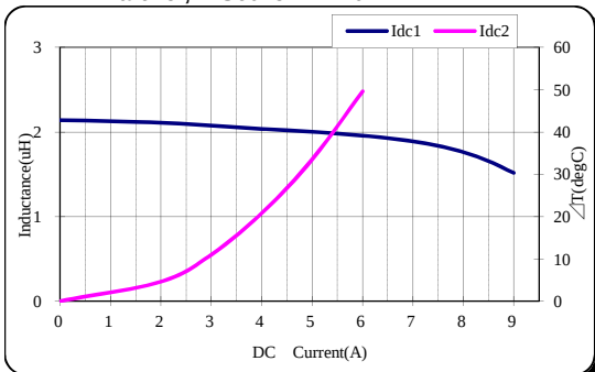
TDK' PartNo.;VLS6045EX-2R0N
