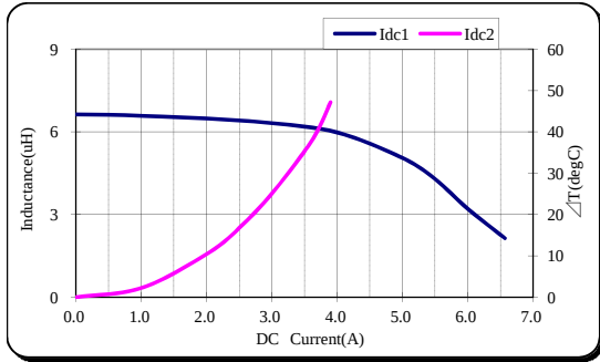
TDK' PartNo.;VLS6045EX-6R8M
