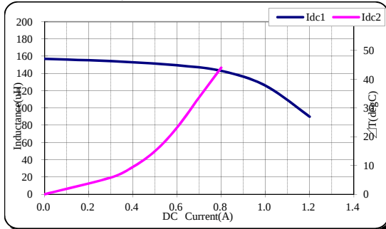
TDK' PartNo.;VLS6045EX-151M
