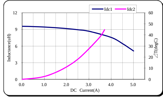
TDK' PartNo.;VLS6045EX-100M
