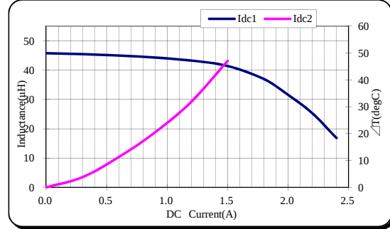
TDK' PartNo.;VLS6045EX-470M
