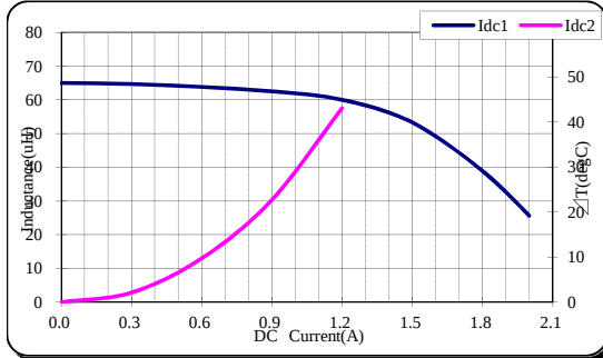
TDK' PartNo.;VLS6045EX-680M
