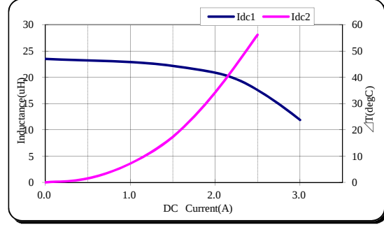
TDK' PartNo.;VLS6045EX-220M
