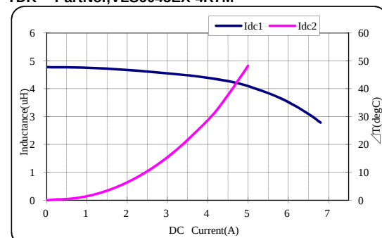
TDK' PartNo.;VLS6045EX-4R7M
