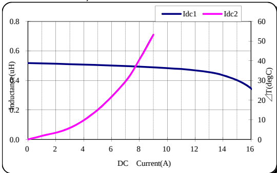
TDK' PartNo.;VLS6045EX-1R2N
