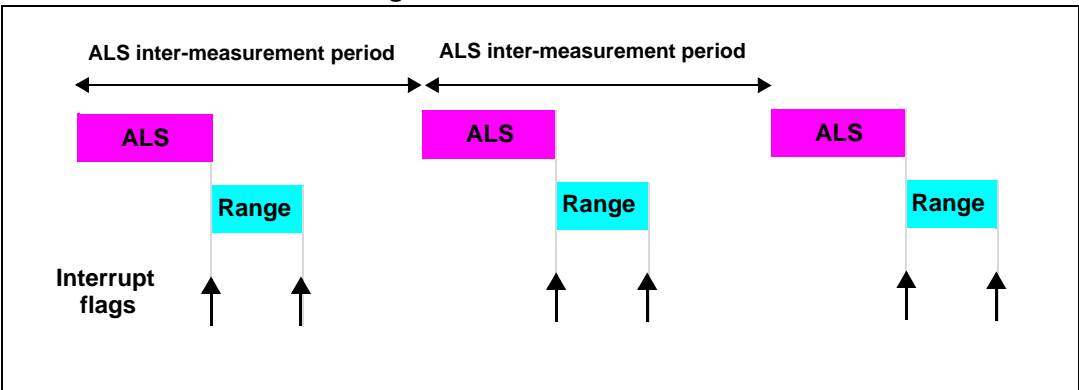
Figure 19. Interleaved mode
