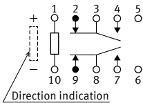
Schematic (BOTTOM VIEW) Single side stable (De-energize)
