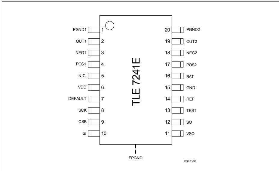
Figure 3 Pin-Out
