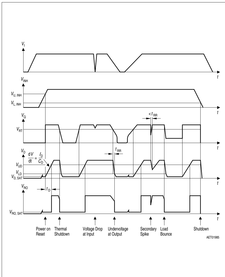
Figure 6 Time Response
