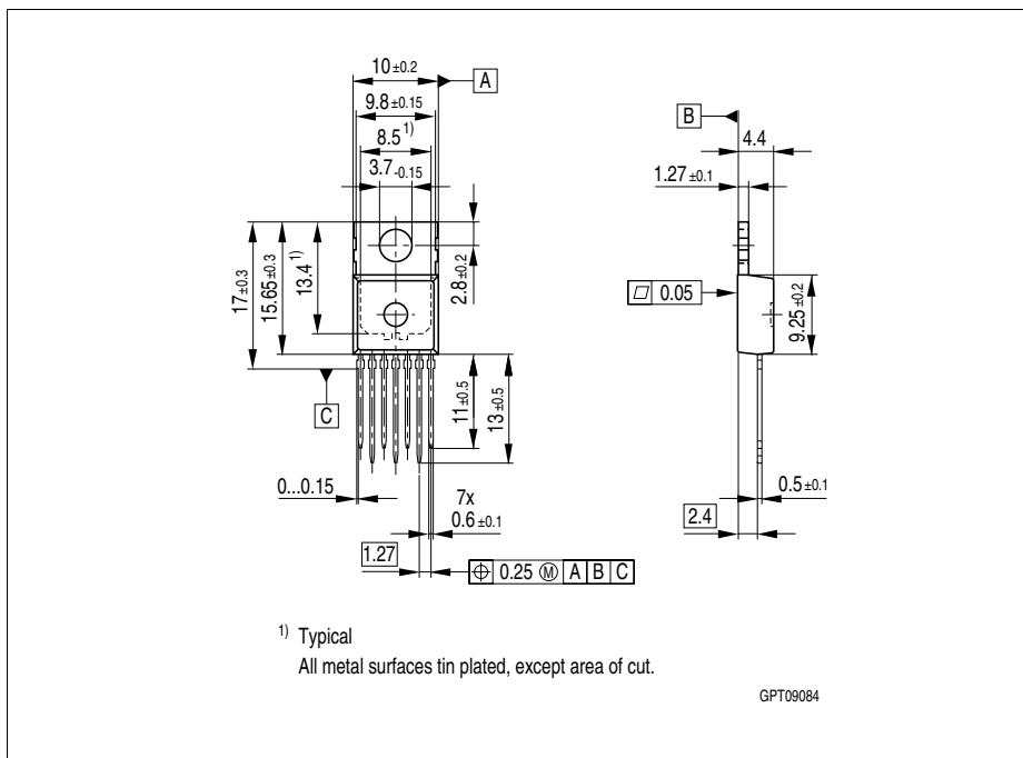
Figure 10 PG-TO220-7-12 (Plastic Transistor Single Outline)
