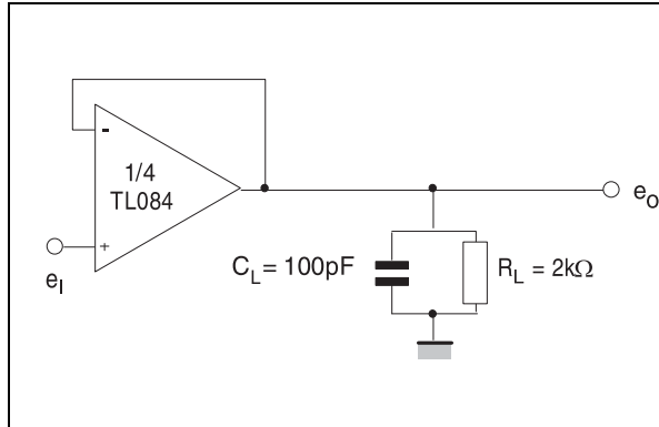
Figure 19. Voltage follower
