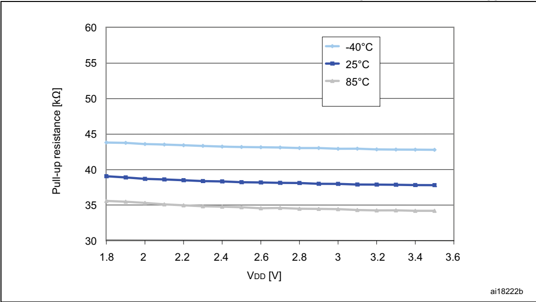
Figure 28. Typical pull-up resistance R_{PU} vs. V_{DD} with V_{IN}=V_{SS}
