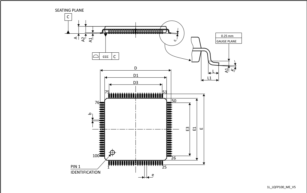
Figure 34. LQFP100 outline
