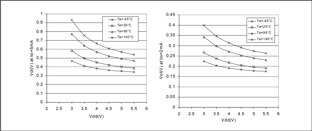
Figure 75. Typical V_{OL} vs. V_{DD} (standard ports)
