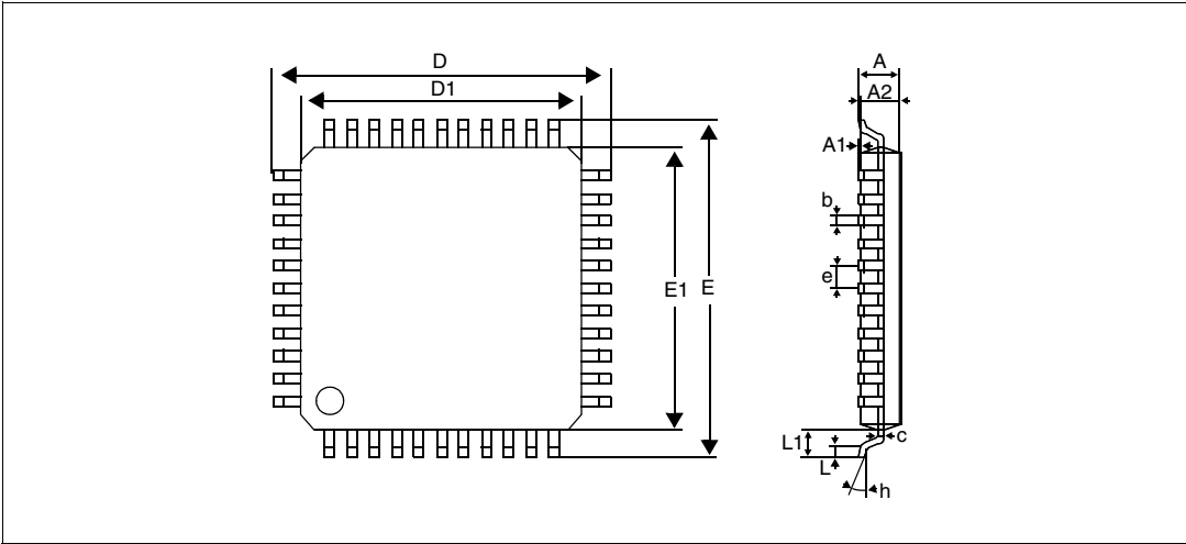
Figure 89. 44-pin low profile quad flat package outline
