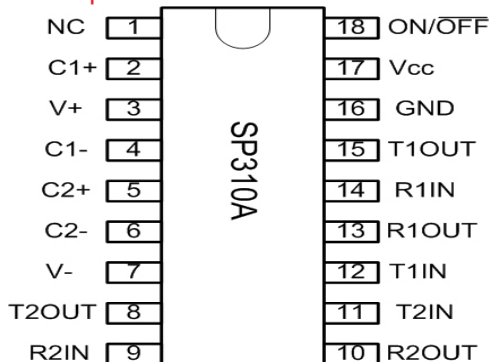
18 pin WSOIC
