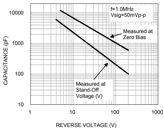
Fig4. Junction Capacitance
