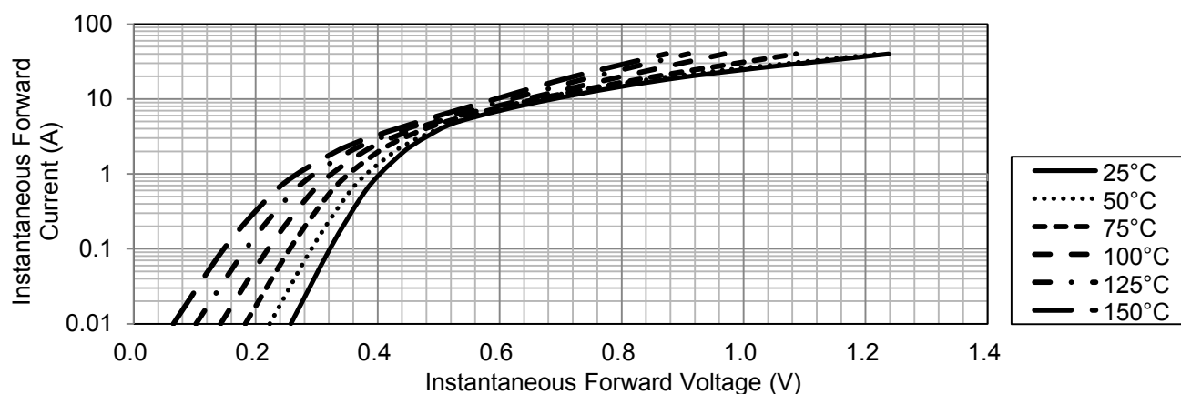
Figure 3. Typical Instantaneous Forward Characteristics (SK32B thru SK34B)
