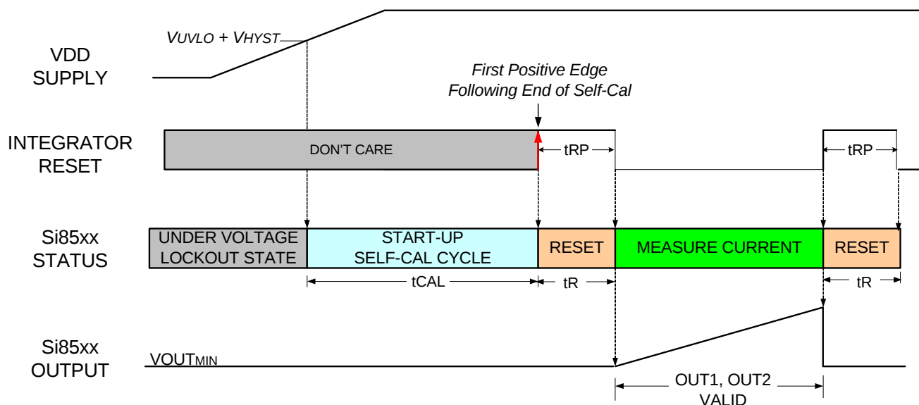
Figure 4. Si85xx Startup and Control Timing
