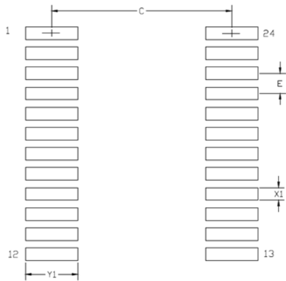
Figure 7. PCB Land Pattern
