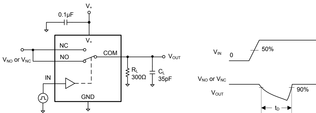
Test Circuit 3. Break-Before-Make Time Delay, t_D
