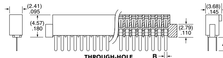
THROUGH-HOLE
