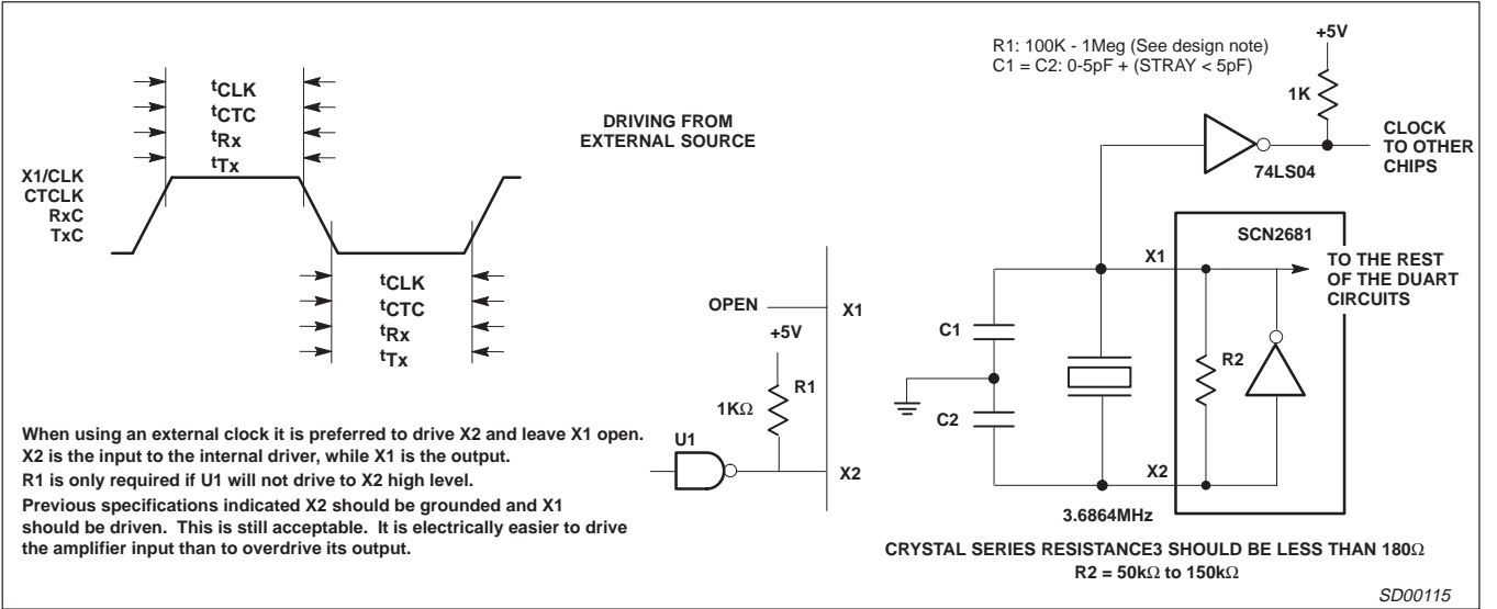
Figure 9. Clock Timing
