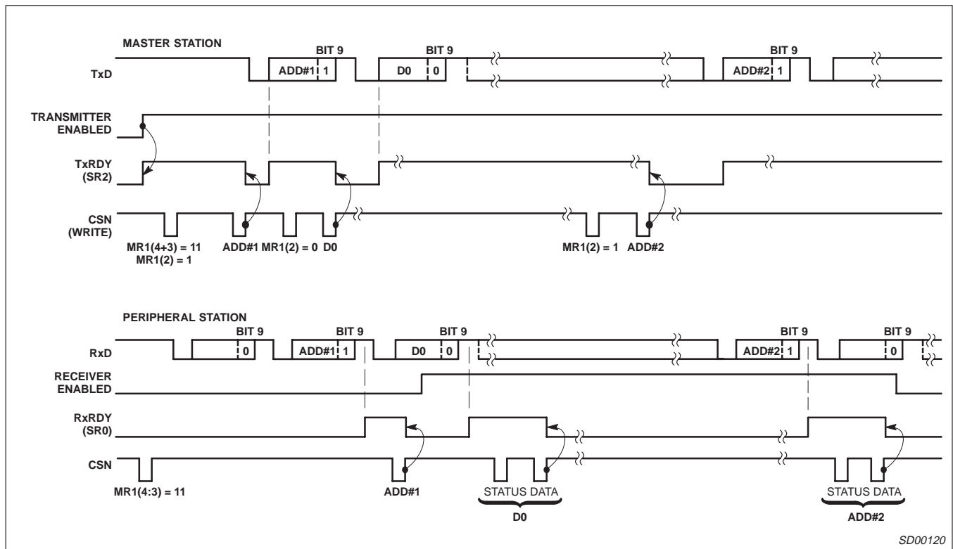
Figure 15. Wake-Up Mode
