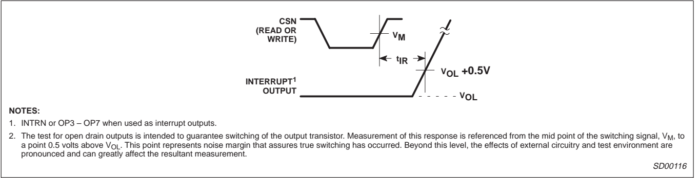
Figure 10. Interrupt Timing
