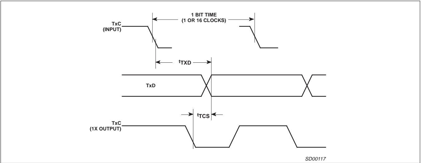
Figure 11. Transmit Timing
