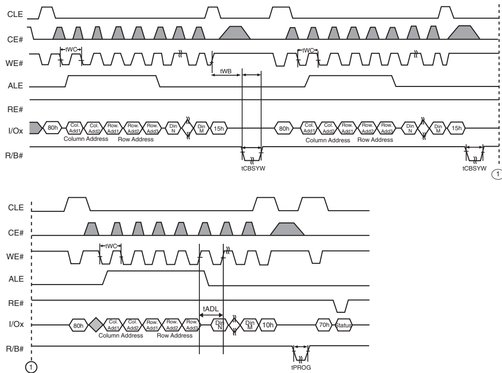
Figure 43. Cache Program
