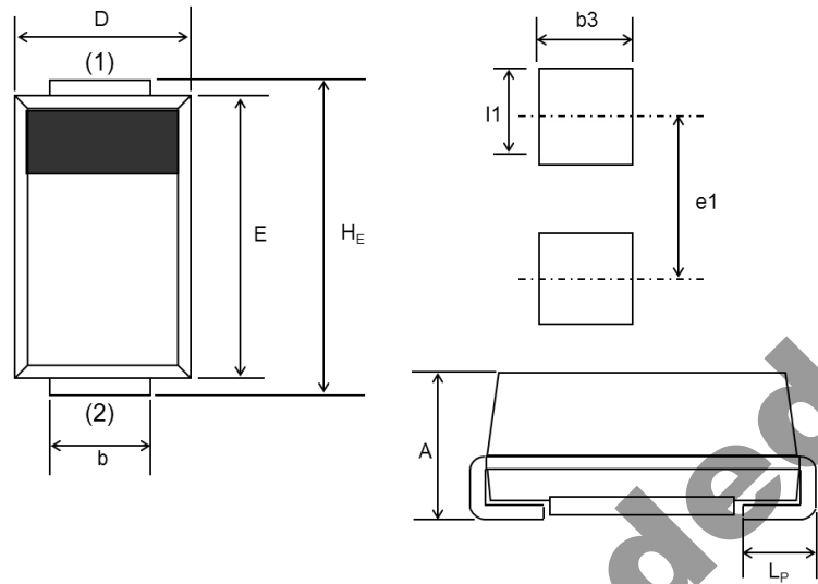
DO-214AC(SMA), (FVDS)
