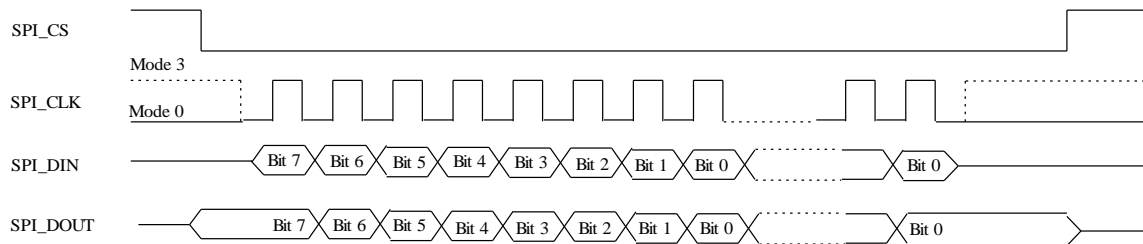
Figure 8: SPI Protocol
