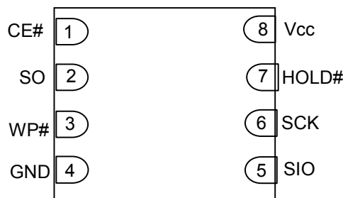
8-Contact WSON
