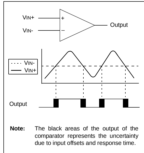
FIGURE 7-1: SINGLE COMPARATOR
