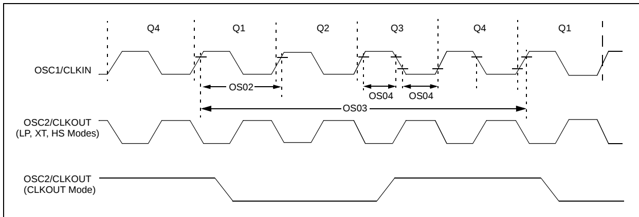
FIGURE 14-4: CLOCK TIMING
