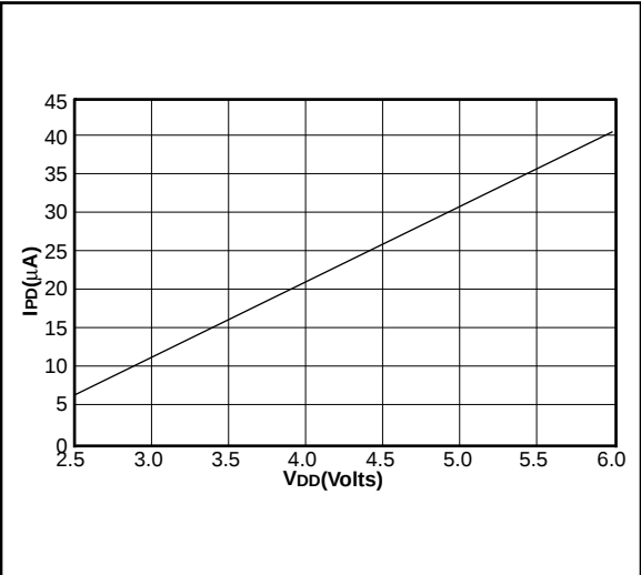
FIGURE 21-11: MAXIMUM I_{PD} vs. TIMER1 ENABLED (32 kHz, RC0/RC1 = 33\text{ pF}/33\text{ pF} , 85°C TO -40°C, RC MODE)
