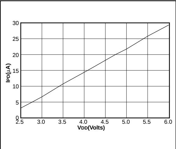
FIGURE 21-11: MAXIMUM I_{PD} vs. TIMER1 ENABLED (32 kHz, RC0/RC1 = 33\text{ pF}/33\text{ pF} , 85°C TO -40°C, RC MODE)
