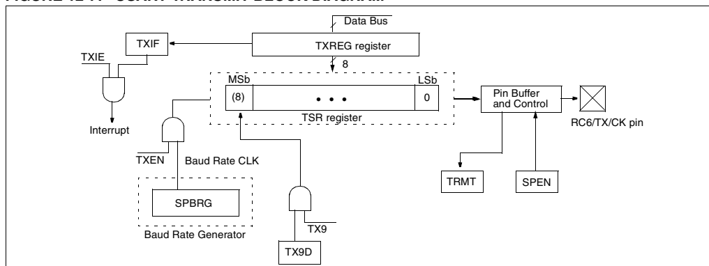
FIGURE 12-7: USART TRANSMIT BLOCK DIAGRAM
