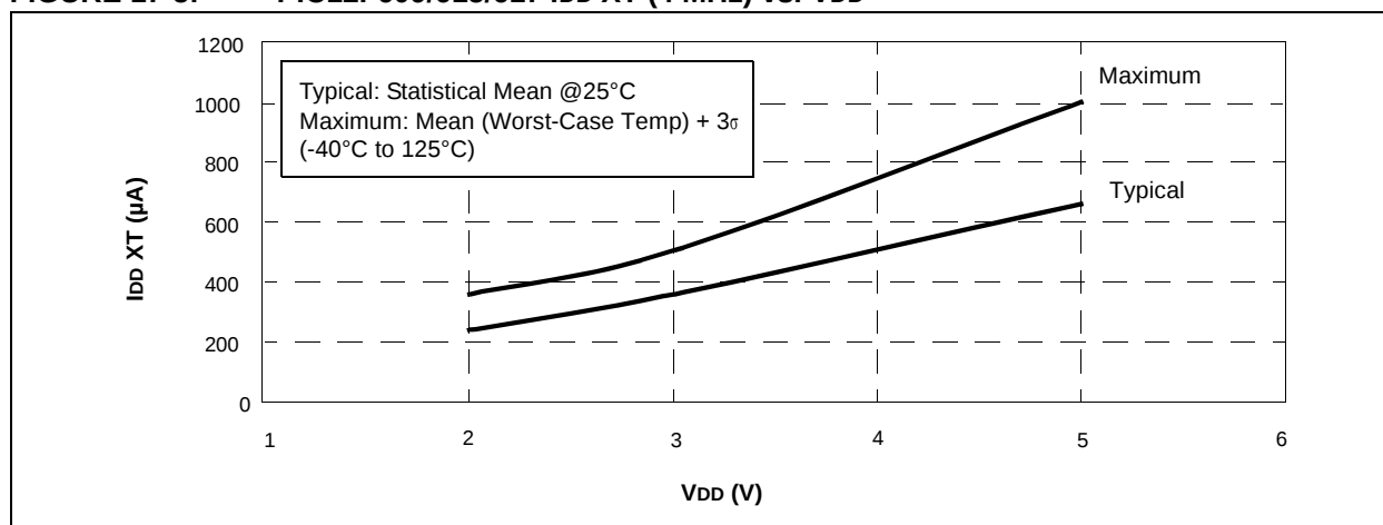
FIGURE 17-5: PIC12F609/615/617 I_{DD\ XT} (4 MHz) vs. V_{DD}
