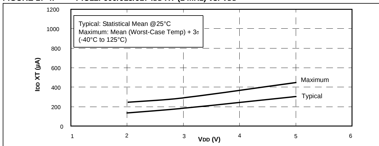
FIGURE 17-4: PIC12F609/615/617 I_{DD\ XT} (1 MHz) vs. V_{DD}
