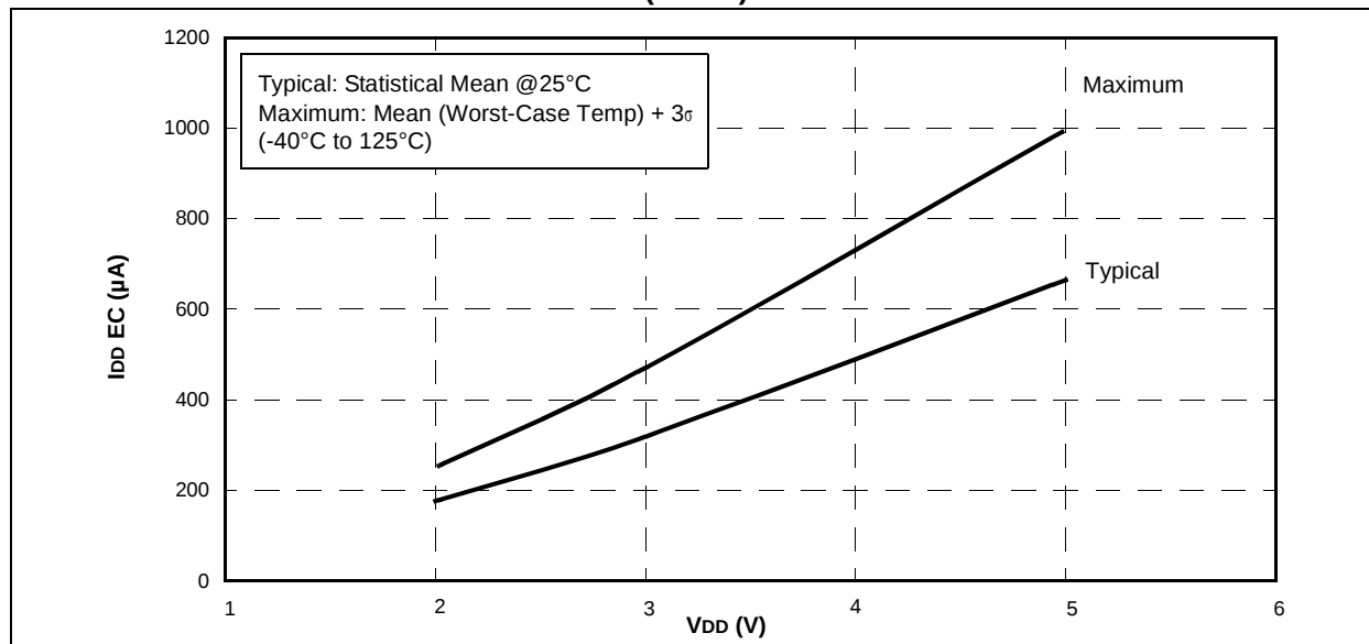
FIGURE 17-3: PIC12F609/615/617 I_{DD\ EC} (4 MHz) vs. V_{DD}
