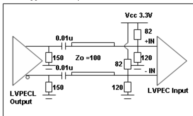
LVPECL Output AC Thevenin Termination
