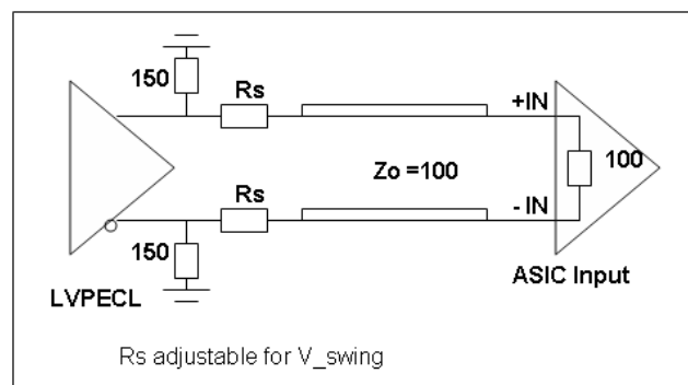
LVPECL V swing Adjustment using Rs
