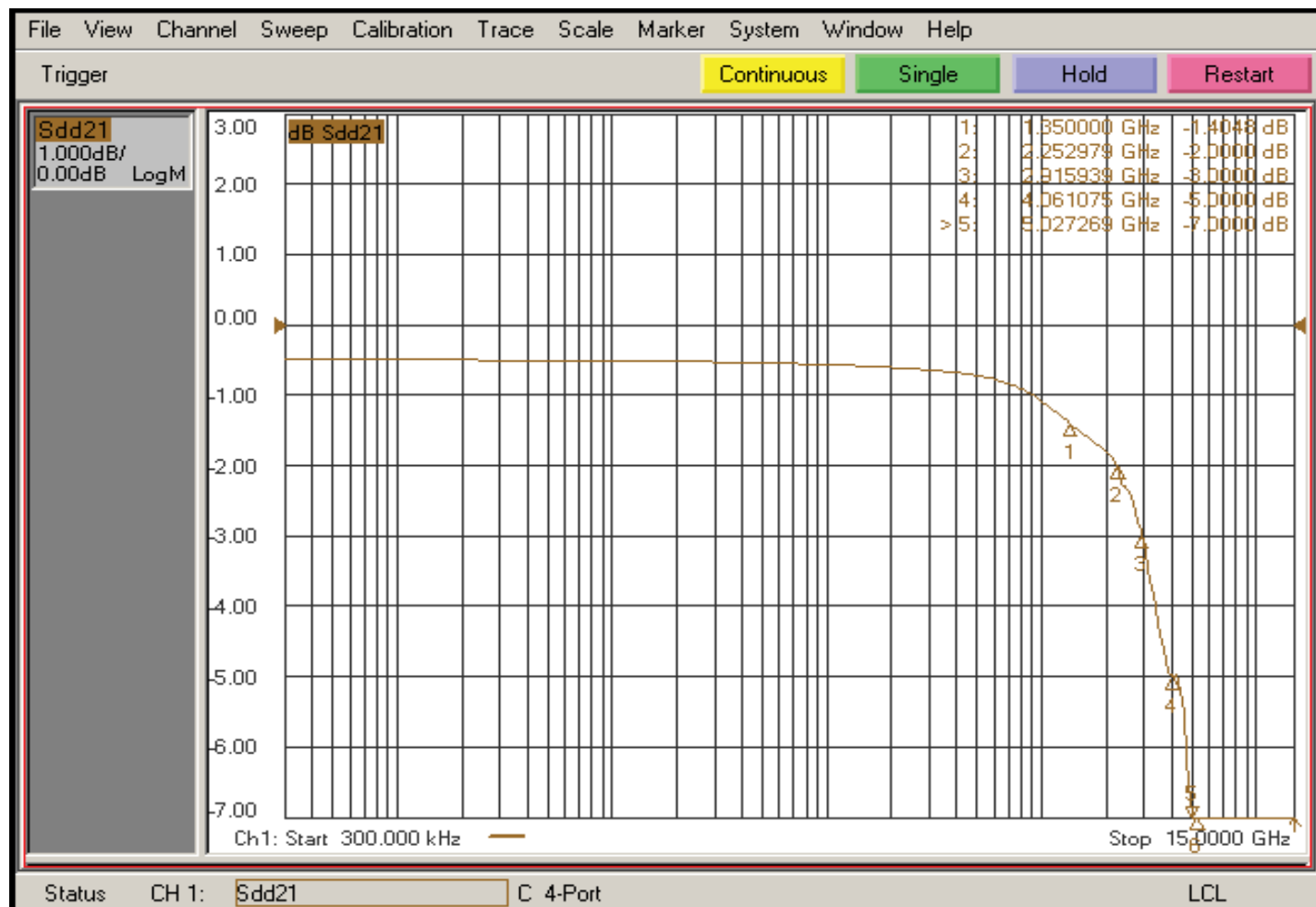
Fig 6. Insertion Loss
