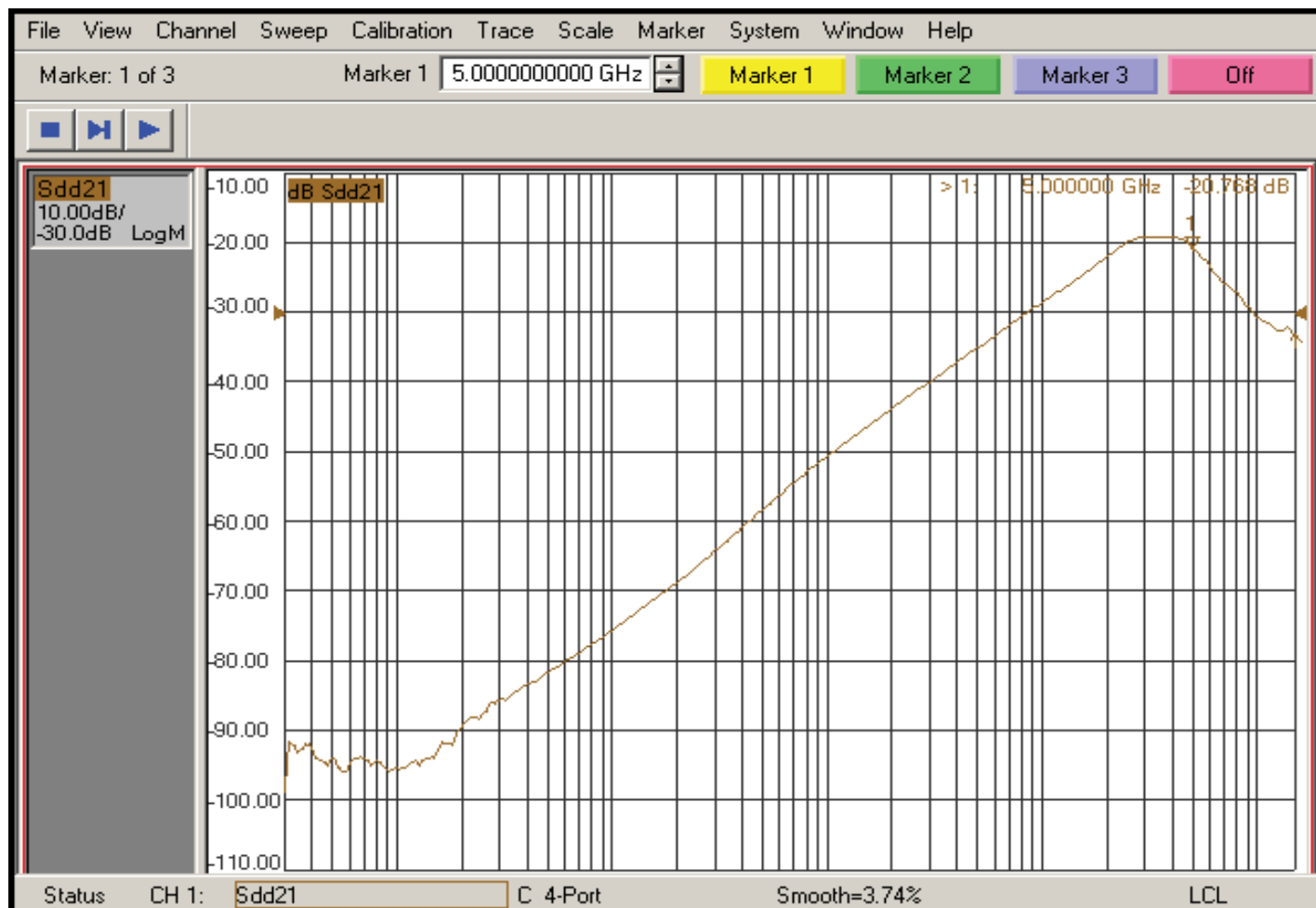
Fig 5. Off Isolation
