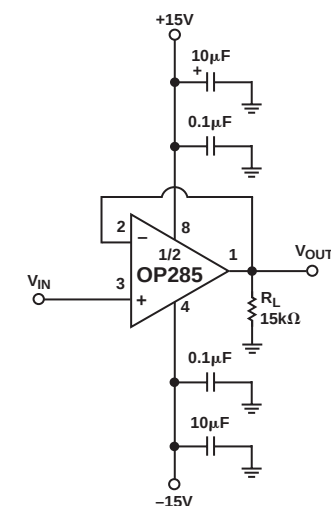
Figure 8. Unity Gain Follower
