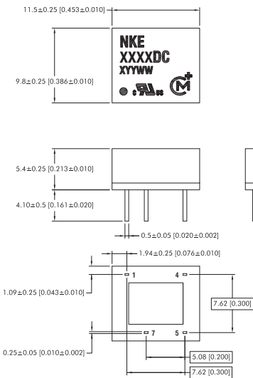
DIP Package
