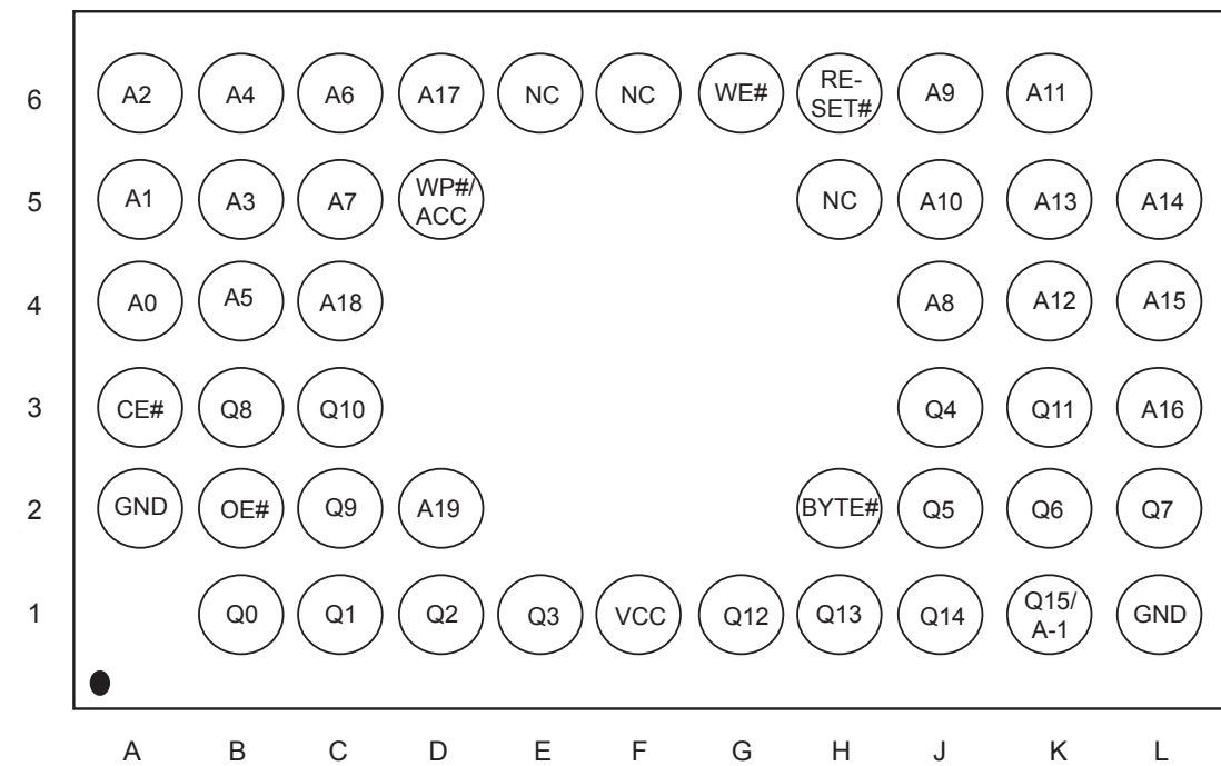
48-Ball XFLGA (Balls Facing Down, 4 x 6 x 0.5 mm)
