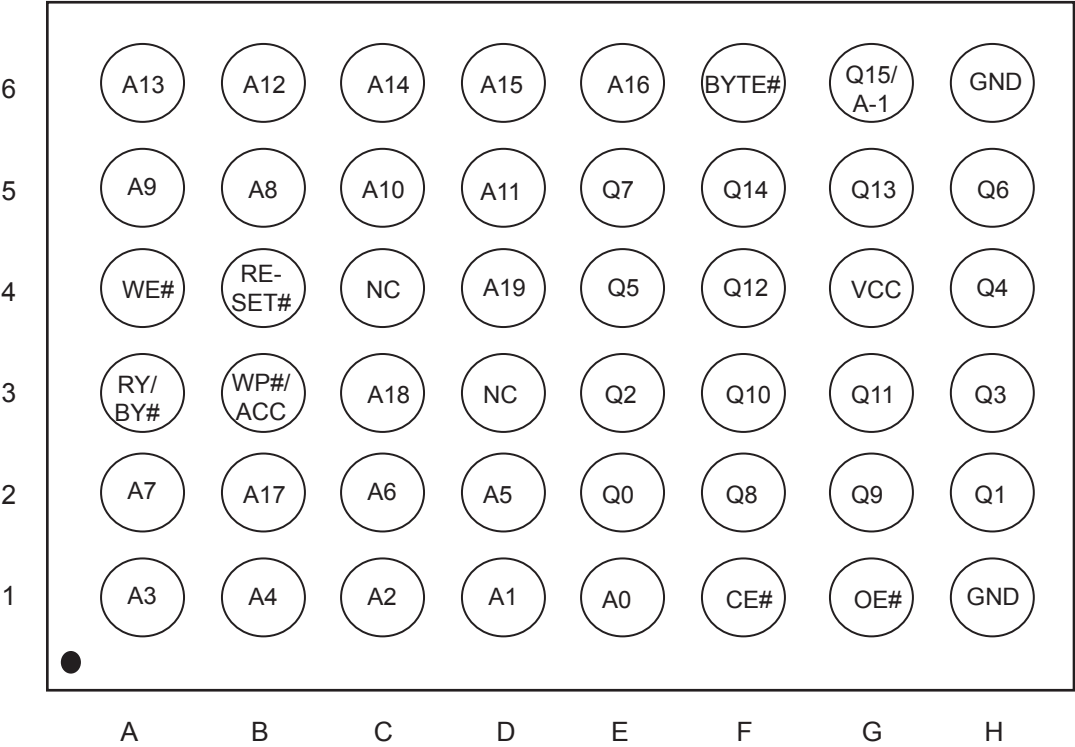
48-Ball CSP(TFBGA/LFBGA) (Ball Pitch = 0.8 mm, Top View, Balls Facing Down, 6 x 8 mm)
