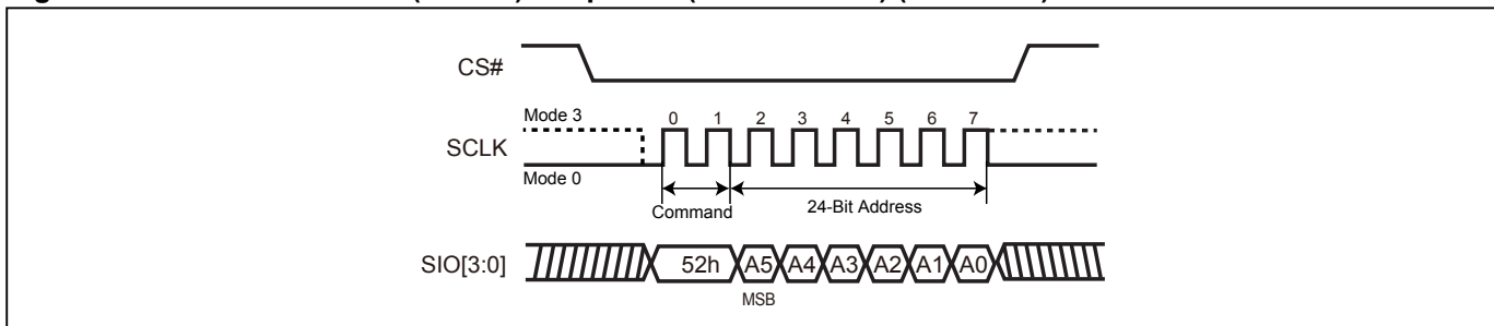
Figure 45. Block Erase 32KB (BE32K) Sequence (Command 52) (QPI Mode)
