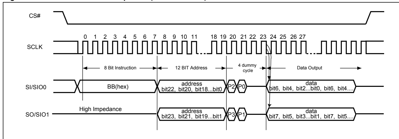
Figure 17. 2 x I/O Read Mode Sequence (Command BB)
