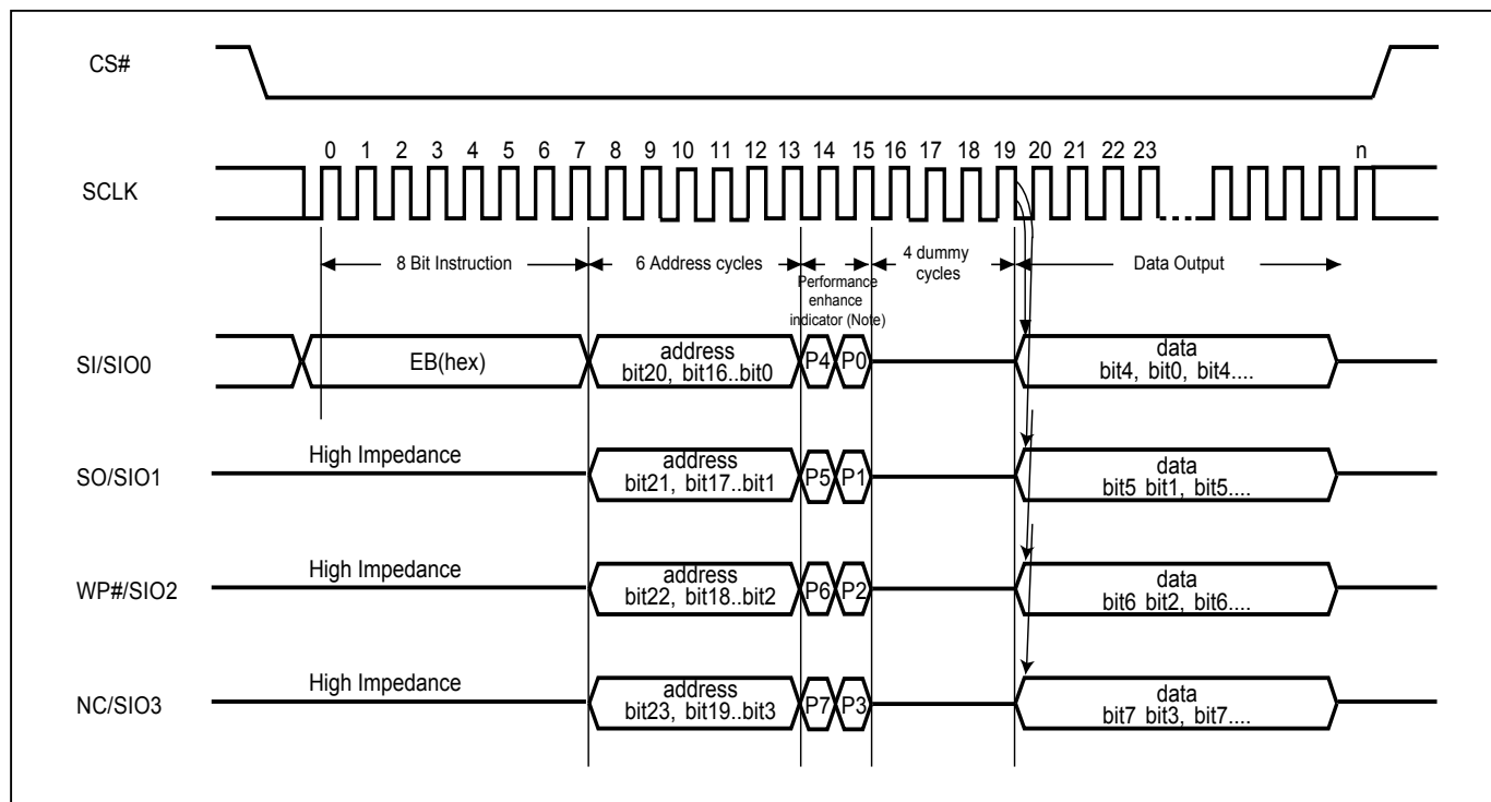
Figure 18. 4 x I/O Read Mode Sequence (Command EB)
