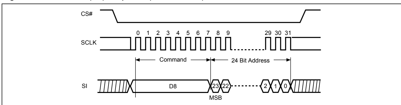
Figure 23. Block Erase (BE) Sequence (Command D8)
