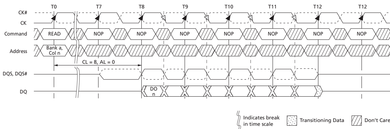
Figure 65: READ Latency
