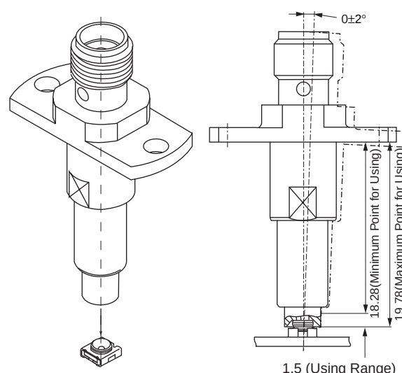
Fig. 1 Insertion the Automatic Measurement Probe (MM126036) in Receptacle (MM8430-2610)
