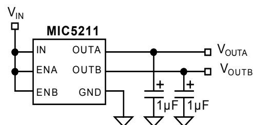
Figure 1. Thermal Conditions Circuit
