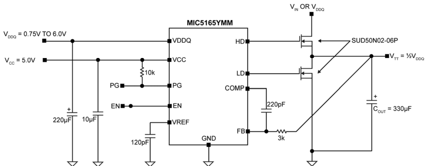
Figure 1. Test Circuit
