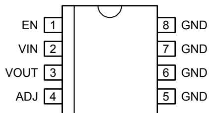
SOIC-8 (M)
