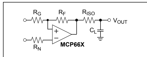
FIGURE 4-6: Output Resistor, R_{ISO} Stabilizes Large Capacitive Loads.
