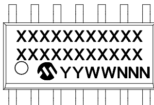
14-Lead SOIC (.150") (MCP660, MCP664)
