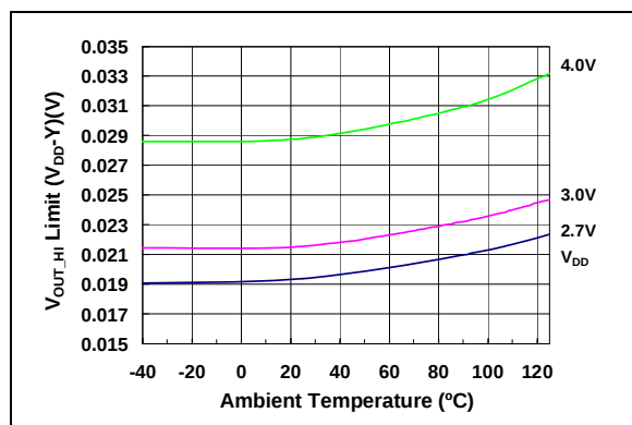
FIGURE 2-25: V_{OUT} High Limit vs. Temperature and V_{DD} .
