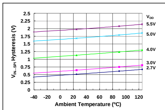
FIGURE 2-24: Input Hysteresis vs. Temperature and V_{DD} .
