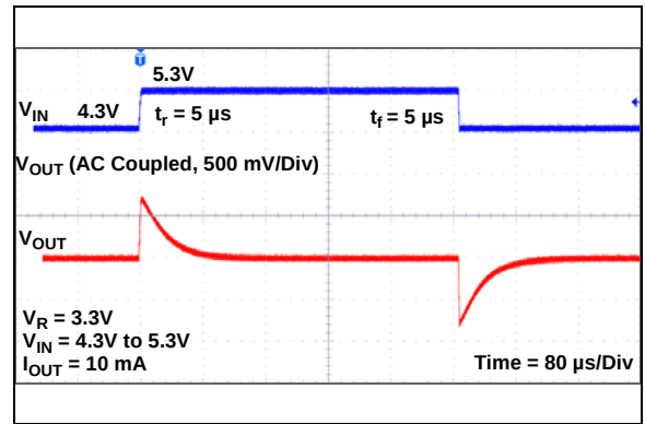
FIGURE 2-46: Dynamic Line Response.
