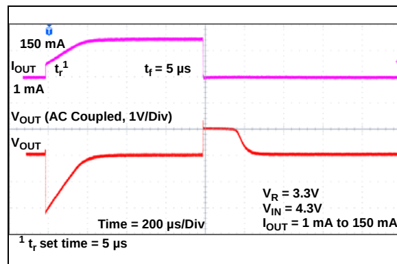
FIGURE 2-60: Dynamic Load Response.
