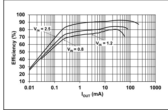
FIGURE 2-5: MCP1624 Efficiency vs. I_{OUT} , V_{OUT} = 3.3V .
