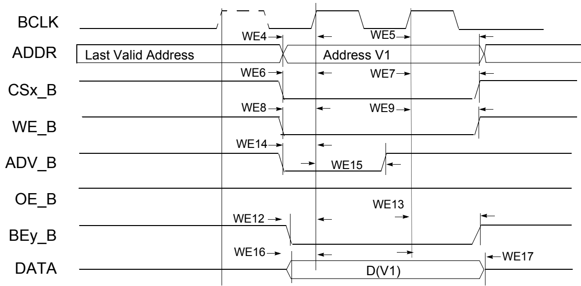
Figure 19. Synchronous Memory, Write Access, WSC=1, WBEA=0, and WADV=0
