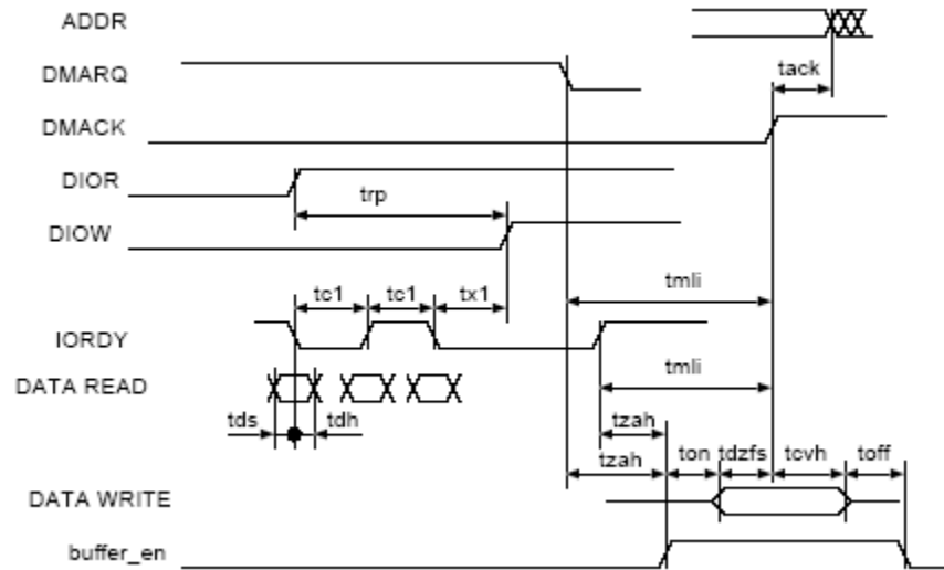
Figure 71. UDMA in Host Terminates Transfer Timing Diagram
