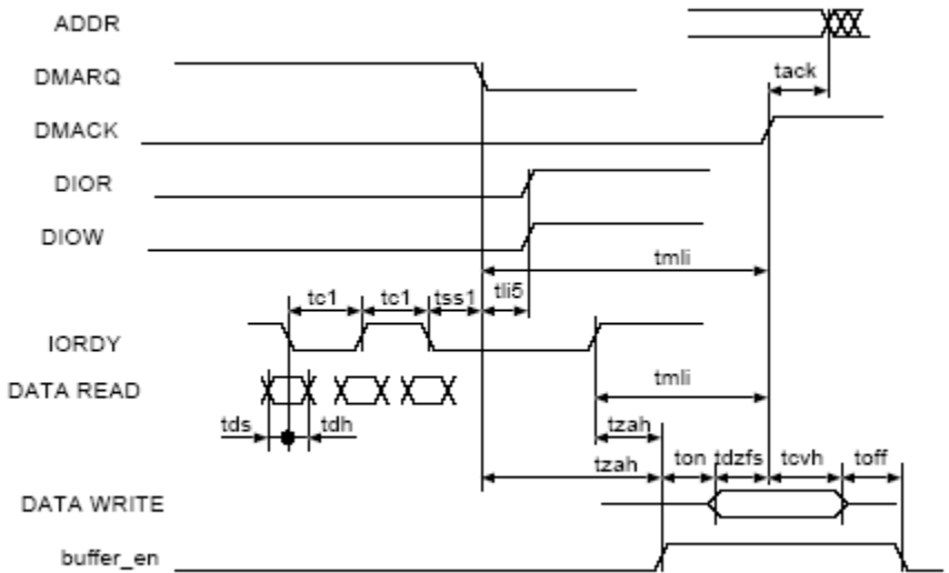
Figure 72. UDMA in Device Terminates Transfer Timing Diagram
