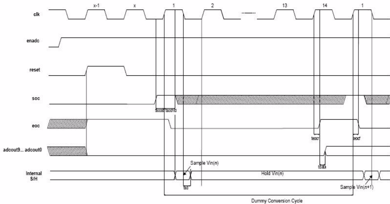
Figure 82. Start-up Sequence
