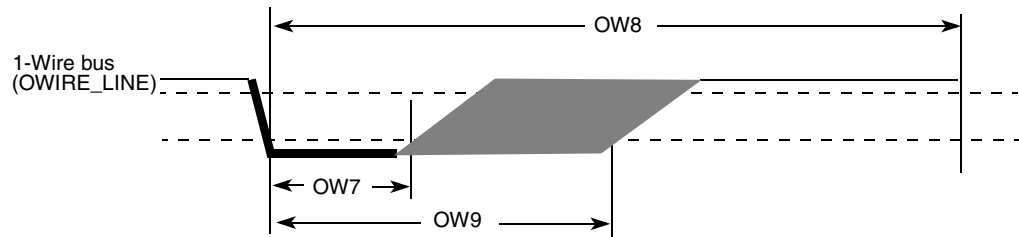
Figure 10. Read Sequence Timing Diagram
