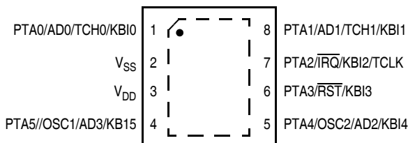
8-PIN ASSIGNMENT MC68HC908QT2 AND MC68HC908QT4 DFN
