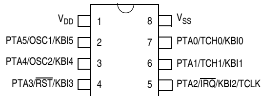
8-PIN ASSIGNMENT MC68HC908QT1 PDIP/SOIC
