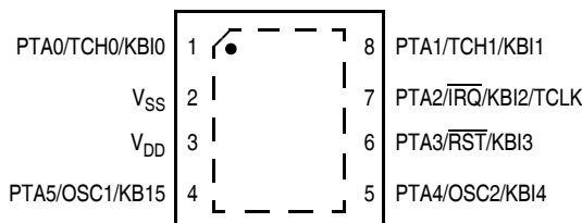
8-PIN ASSIGNMENT MC68HC908QT1 DFN
